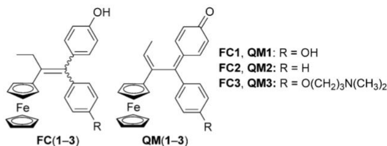
Figure 1. Ferrociphenols used as substrates in this study and their corresponding quinone methides (wavy-line bonds indicate the presence of both cis and trans isomers at the level of the double bond).
