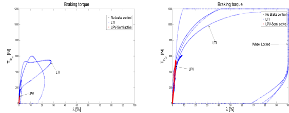
Fig. 11: Rear right Break- Fig. 12: Rear left Breaking ing torque.
