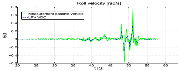
Fig. 17: Roll velocity of the chassis \dot{\theta}
