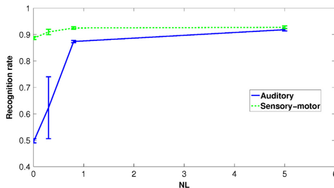
Fig. 10. Recognition rate as a function of the nonlinearity strength NL , at the end of simulations of auditory and sensory–motor agents. Ten independent simulations were run for each condition, from which means and standard deviations were computed. Each involved four agents and two objects. In all simulations, \sigma_{Env} was set to a rather high value (5), and \sigma_{Ag} was set to a low value (0.1).
