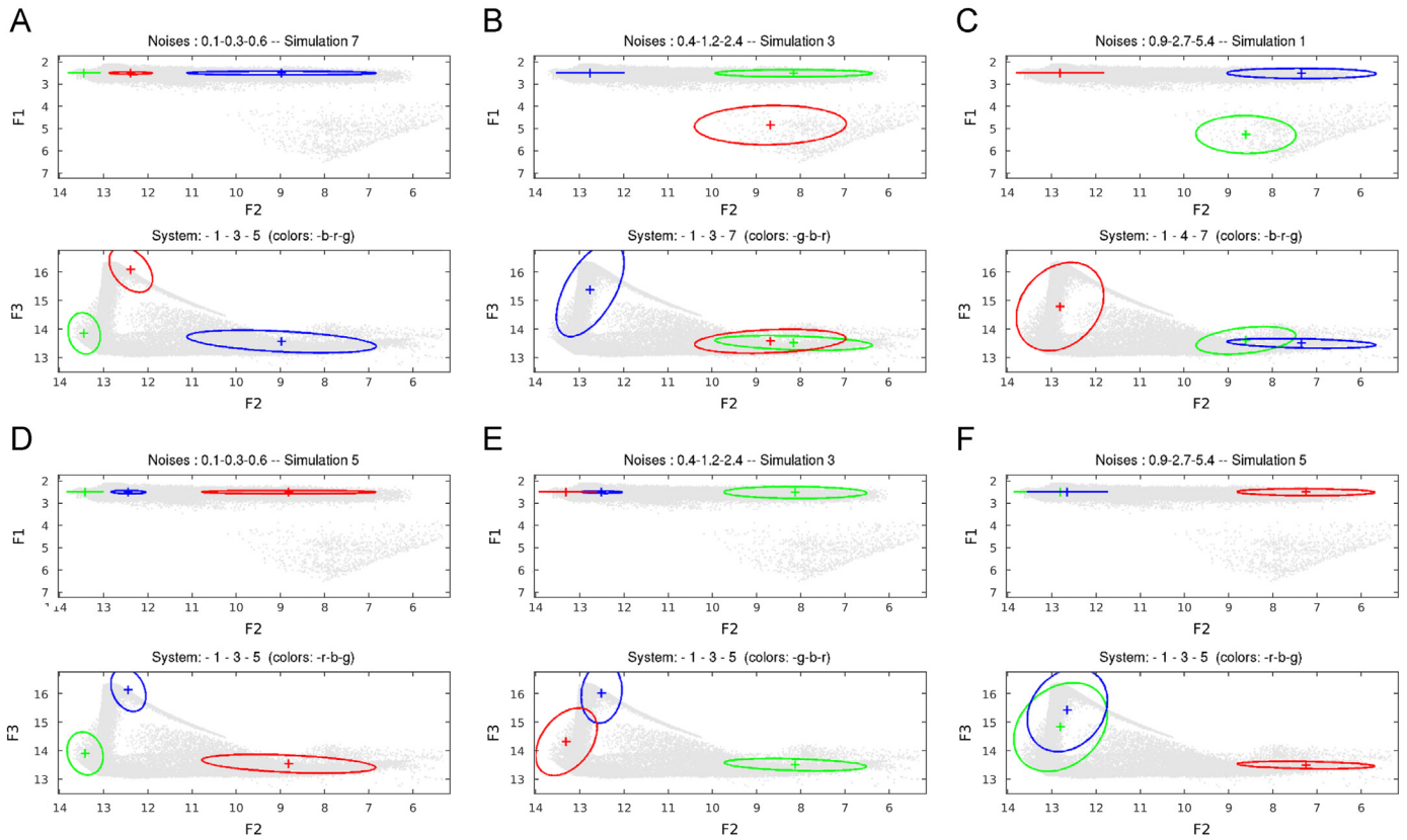
Fig. 17. Typical systems obtained in stop simulations. Same convention as in Fig. 13 B. Top line (A, B, C): “free-jaw” simulations. Bottom line (D, E, F): “high-jaw” simulations. Left column (A, D): low noise level, with \sigma_{F1} = 0.1, \sigma_{F2} = 0.3, \sigma_{F3} = 0.6 . Center column (B, E): medium noise level, with \sigma_{F1} = 0.4, \sigma_{F2} = 1.2, \sigma_{F3} = 2.4 . Right column (C, F): high noise level, with \sigma_{F1} = 0.9, \sigma_{F2} = 2.7, \sigma_{F3} = 5.4 .
