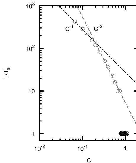
FIG. 7: Period of navigation as a function of confinement C . \Gamma = 0.085 . Circles (diamonds) correspond to symmetric (asymmetric) motion of the swimmer.
