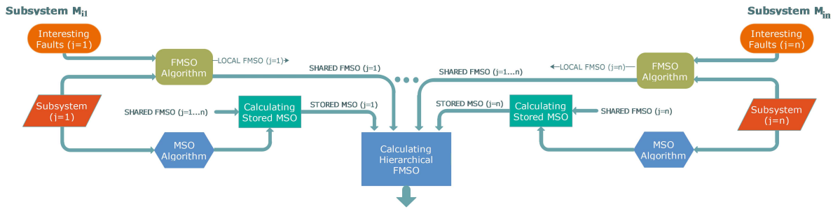
Figure 2. Architecture of diagnoser offline
