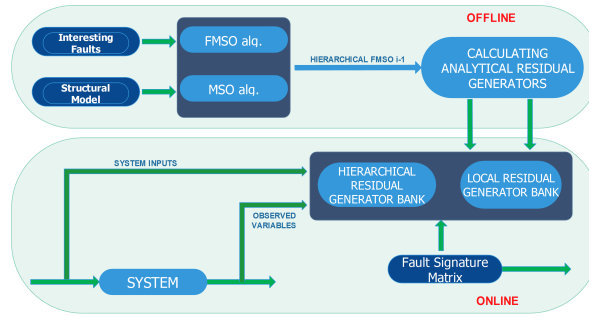
Figure 3. Scheme of a decentralized diagnoser for a subsystem at level i
