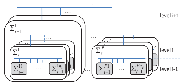
Fig. 2. Generic decentralized diagnosis structure
