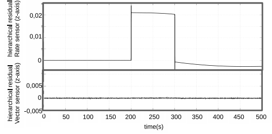
Fig. 15. ADS hierarchical residuals for the z-axis
