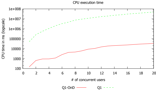
Figure 9: Concurrent query execution
