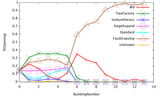
Fig. 8: Evolution of P(\text{Opening}) with increasing observations in a TvP match-up, with Weber’s labeling. The x-axis corresponds to the construction of buildings.
