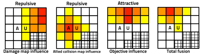
Fig. 4: Simple example of Bayesian fusion from 3 sensory inputs (damages, collisions avoidance, and goal attraction). The grid pattern represents statically occupied terrain, the unit we control is in U, an allied unit is in A. Red represents the highest probabilities, white the lowest. The result is displayed on the rightmost image, where our unit should try and go to the red square.
