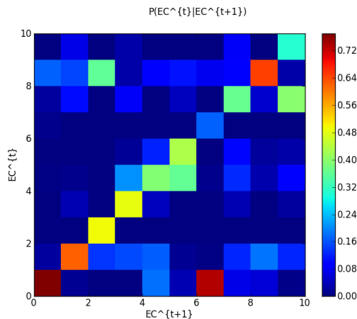
Fig. 10: Dynamics of clusters: P(EC^t | EC^{t+1}) for Zerg, with \Delta t = 2 minutes
