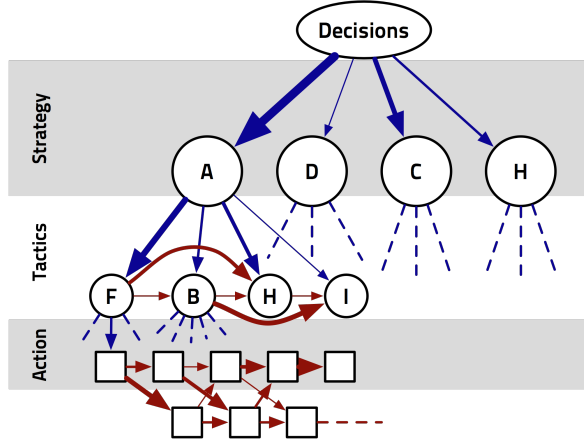
Fig. 1: Sequential (horizontal, red) and hierarchical (vertical, blue) decision constraints. At the strategic level: A, D, C, H respectively stand for attack, defend, collect, hide ; while at the tactical level: F, B, H, I respectively stand for front, back, hit-and-run, infiltrate. The squares correspond to actionable (low level) decisions, like moving a unit or making it attack a target.
