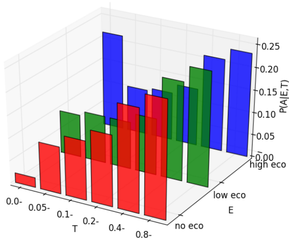
Fig. 5: P(A) for varying values of E and T , summed on the other variables, for Terran in TvT. Zones with no economy are in red bars, with a low economy in green and the principal economy in blue. The main difference along this economical axis comes at the lowest tactical values of regions (for the defender) at T < 0.05 (noted T = 0.0 ) and showcases sneaky attacks to unprotected economical regions.
