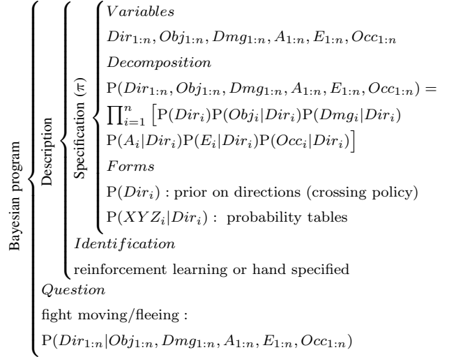
Fig. 3: Bayesian program of the flee() and fightMove() behaviors. This is mainly a Bayesian sensors fusion model.
