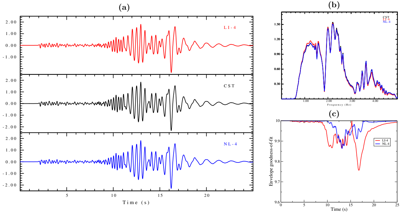
Figure 6. Same as Figure 5 but using N = 4 relaxation mechanisms.
