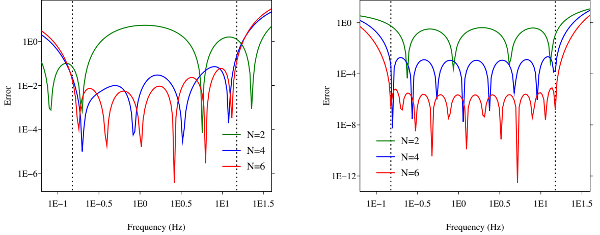
Figure 2. Value of the objective function of Equation (32) as a function of frequency, using a Zener approximation with N = 2 (green curve), N = 4 (blue curve), and N = 6 (red curve) relaxation mechanisms, with the linear approach of Emmerich & Korn (1987) (left) and with nonlinear optimization (right). The vertical dotted lines denote the interval of optimization [f_{\min}, f_{\max}] . Both axes are in logarithmic scale. Note that the vertical logarithmic scale has about twice more decades on the right figure than on the left figure, i.e., the error levels are very significantly different.
