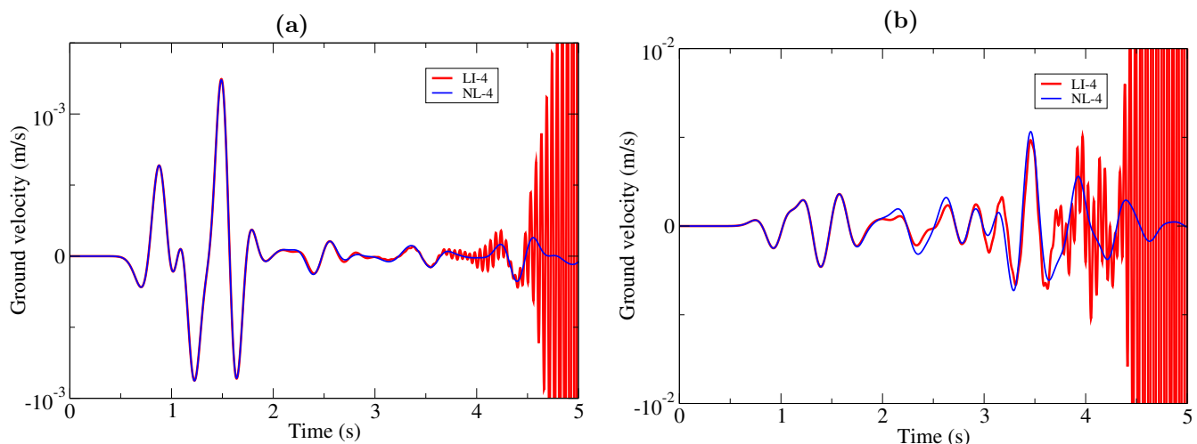
Figure 8. Time evolution of vertical ground velocity computed by the spectral-element method at two surface receivers located (a) 500 m outside and (b) 500 m inside the 2D valley (black triangles in Figure 7). The viscoelastic model of Table 3 is approximated with the Zener model using four relaxation mechanisms obtained based on linear (red) or nonlinear (blue) optimization. In this example the model defined by the linear relaxation coefficients yields an unstable solution.
