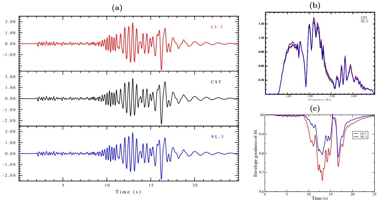
Figure 5. (a) Time evolution of horizontal ground acceleration in \text{cm/s}^2 at 4-km epicentral distance for a constant Q model (black line), and for the Zener model with N = 3 relaxation mechanisms obtained based on linear (red) or nonlinear (blue) optimization. (b) Corresponding Fourier amplitude spectra. (c) Time evolution of the envelope goodness-of-fit with respect to the reference solution of the constant Q model.
