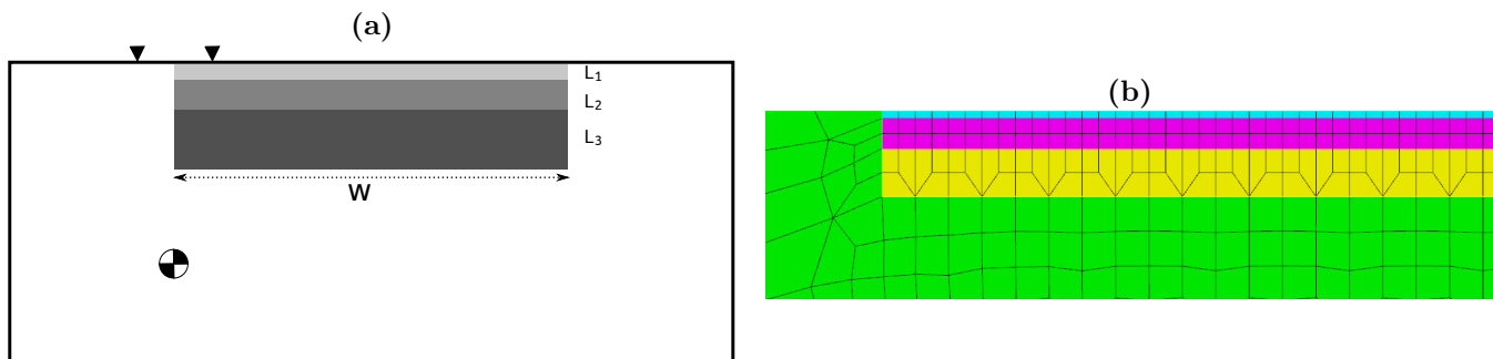
Figure 7. (a) Vertical cross-section (not to scale) of the three-layer-over-a-half-space valley model used in this article. The medium is excited by a double-couple point source whose position is indicated by the beach ball. Two surface receivers, located 500 m inside and outside the valley, are indicated with triangles. The width of the valley is W = 4.5 km. The properties of the three layers are given in Table 3. (b) Close-up on the unstructured, geometrically-conforming spectral-element mesh used to perform the 2D calculations.
