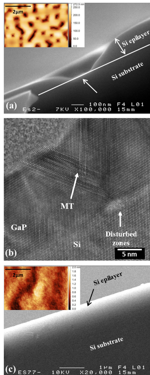
FIG. 1. (a) Cross-sectional SEM image of silicon homoepitaxial layer grown on the Si substrate cleaned by modified RCA process. Insetted AFM image shows high r.m.s. surface roughness (48 nm); (b) HRTEM images of a GaP epilayer grown on the Si substrate cleaned by modified RCA process; (c) cross-sectional SEM image of silicon homoepitaxial layer grown on the Si substrate cleaned by optimized HF cleaning process. The r.m.s. roughness measured on insetted AFM image is about 0.3 nm.
