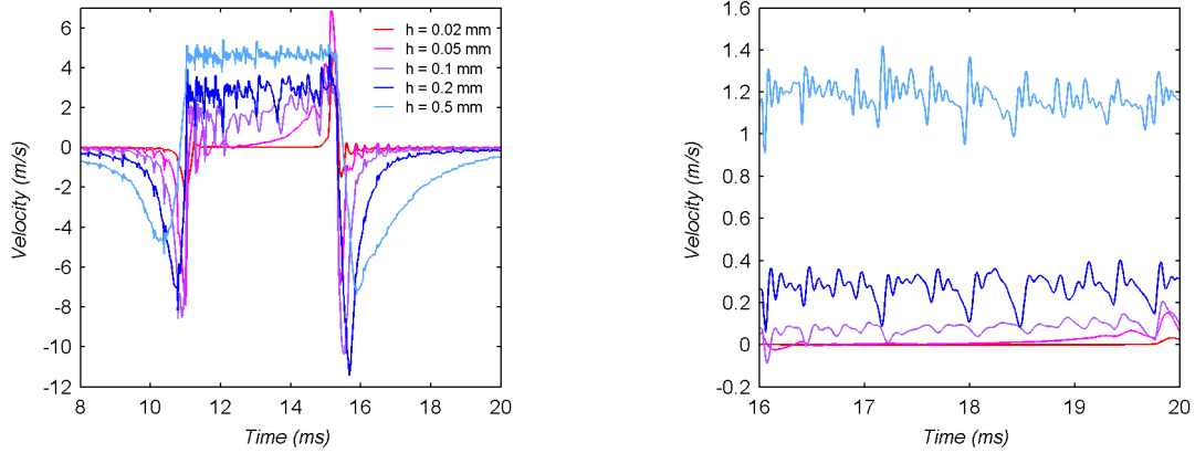
(a) Flow velocities v in the channel
