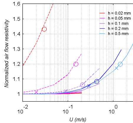
(b) Normalized air flow resistivity calculated for incompressible flow (-) and compressible flow (--). (x) and (o) stand for respectively the values in average and maximum flow conditions during the tyre rolling calculated in section 3.2
