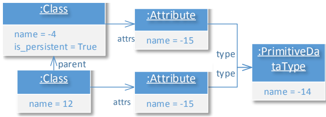
Fig. 7. Excerpt of an input model transformed into an incorrect output model (whose an excerpt is illustrated Figure 6)
