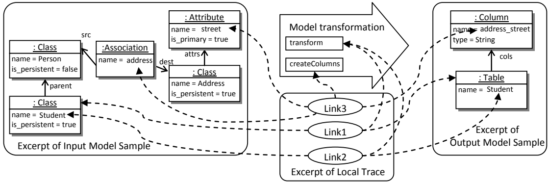
Fig. 8. Example of a trace between one input class model and its corresponding rdbms model
