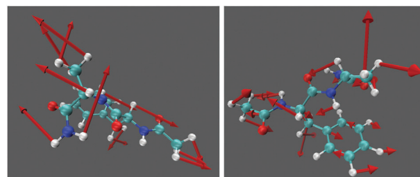
Fig. 11 Assignments from DMD calculation for 1599 \text{cm}^{-1} normal mode defined as \text{CH}_3 umbrella and \text{NH}_2 bending (left) and 1465 \text{cm}^{-1} (right) normal mode for \text{C}-\text{H} bend contributions.
