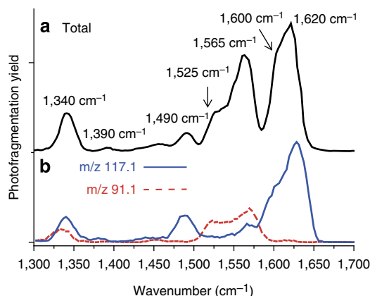
Figure 5 | Total and mass-resolved IRMPD spectra from m/z = 145.1 ion. a shows the experimental IRMPD spectrum (black straight line) of the m/z = 145.1 ion in the 1,300\text{--}1,700\text{ cm}^{-1} range. Mass-resolved IRMPD spectra are shown in b. Two fragmentation channels are detected at m/z = 117.1 (straight blue line) and at m/z = 91.1 (dotted red line).
