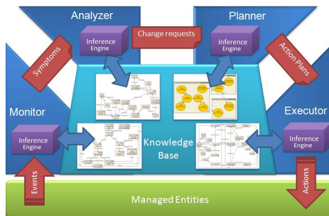
Figure 1. FRAMESELF architecture overview
