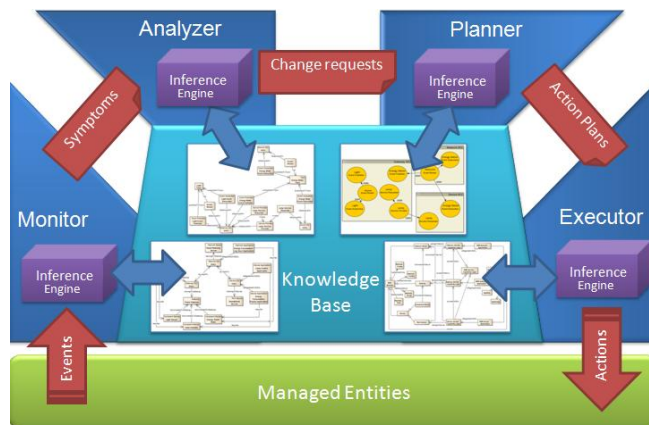
Figure 1. FRAMESELF architecture overview
