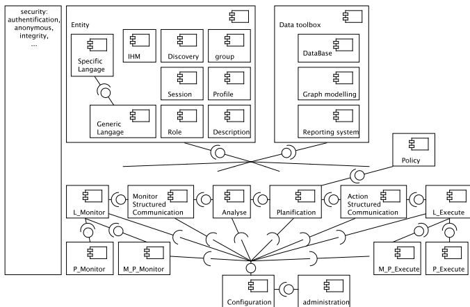
Figure 1. Framework architecture
