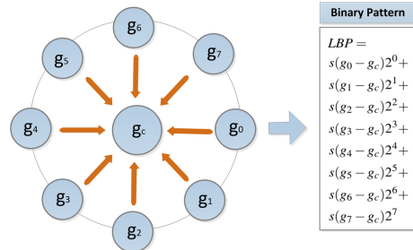
Figure 2: The LBP descriptor.
