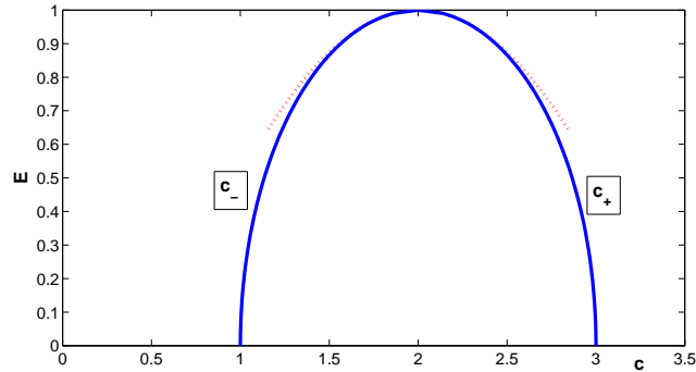
Figure 2: The values c_{\pm} given by the explicit expressions (1.13) are represented as a function of the parameter \mathcal{E} (solid line). The asymptotic result (1.12) is shown by dashed lines.
