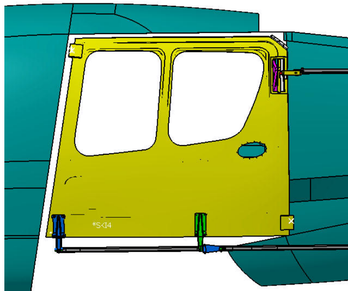
Figure 3, Door linkage devices.
