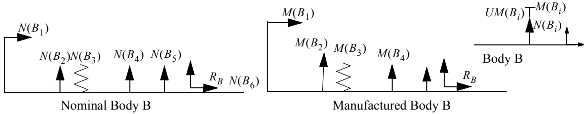
Figure 2: Manufactured component
