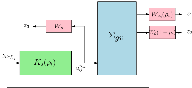
Fig. 3. Suspension system generalized plant.
