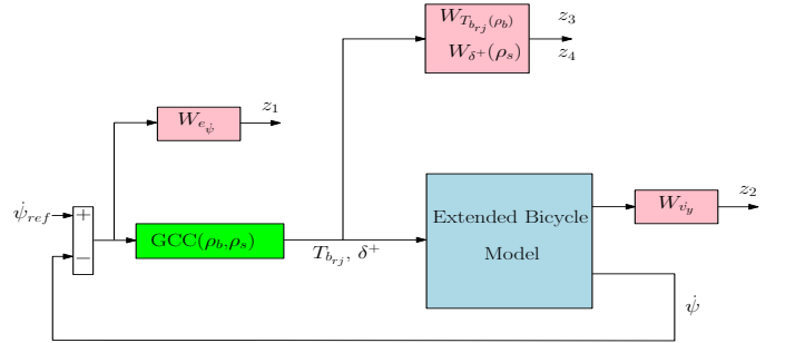
Fig. 2. Generalized plant for braking/steering control synthesis.
