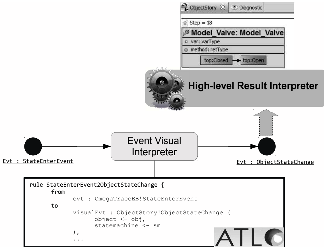
Fig. 4. Graphical rendering of high-level events. The Event Visual Interpreter executes a model transformation to generate the input model for the visual renderer.
