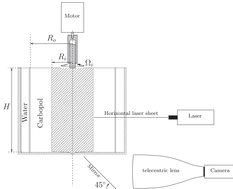
Fig. 2. Sketch of the experimental set-up.
