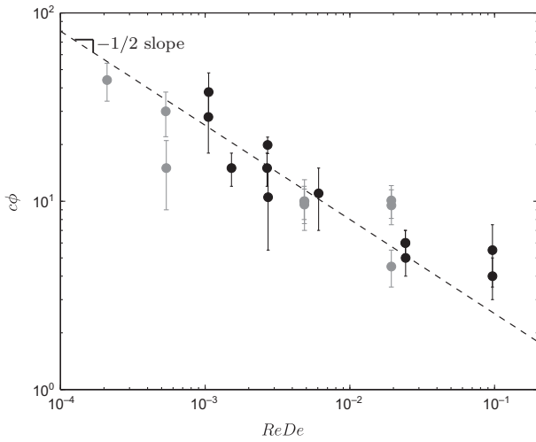
Fig. 11. Velocity of the propagating elastic front c_\phi as a function of ReDe for Carbolpol A (black dots) and Carbolpol B (gray dots). The dotted line corresponds to a (ReDe)^{-1/2} law.
