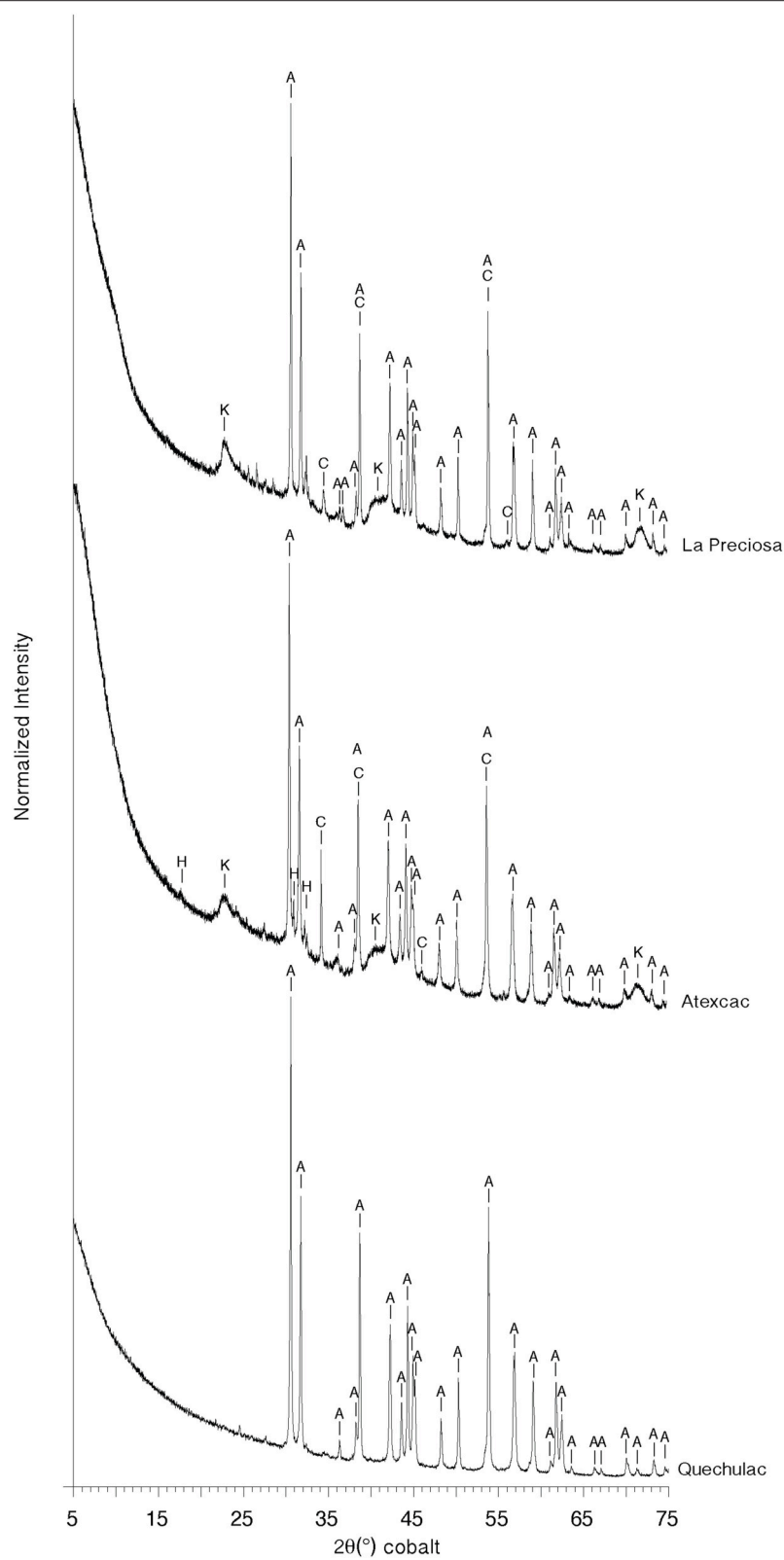
FIGURE 2 | Bulk X-ray diffraction patterns for La Preciosa, Atexcac, and Quechulac microbialite samples. Aragonite (A), calcite (C), and a kerolite phase (K) are identified from the XRD pattern of La Preciosa microbialite. Aragonite (A), calcite (C), hydromagnesite (H), and kerolite (K) can be identified from the Atexcac XRD pattern. Only aragonite (A) can be identified in the Quechulac microbialite XRD pattern.
