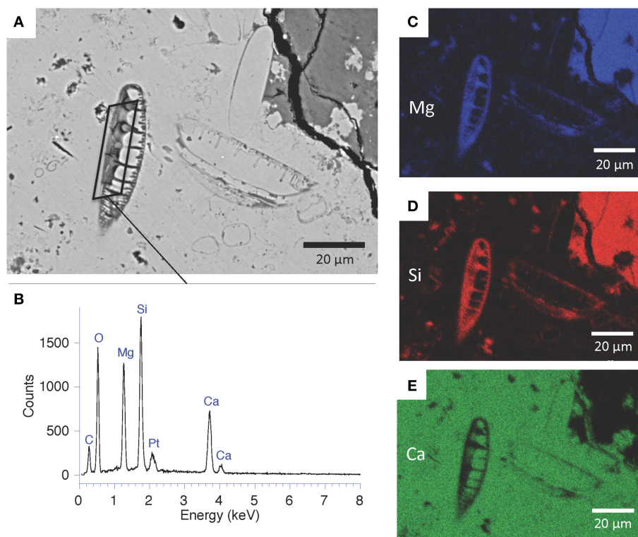
FIGURE 6 | SEM analyses of fossil diatoms enclosed in Ca-carbonate and replaced by kerolite in Atexcac microbialite. (A) SEM micrograph in the backscattered electron mode. Two diatom frustules can be recognized in the center of the image; (B) SEM-EDXS spectrum of the area outlined in (A) . Platinum was deposited to conduct surface charges upon observations; (C–E) EDXS maps of magnesium, silicon, and calcium showing two diatoms replaced by a Mg-silicate phase.
