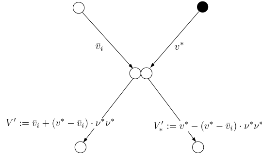
FIGURE 18. Scattering relations
