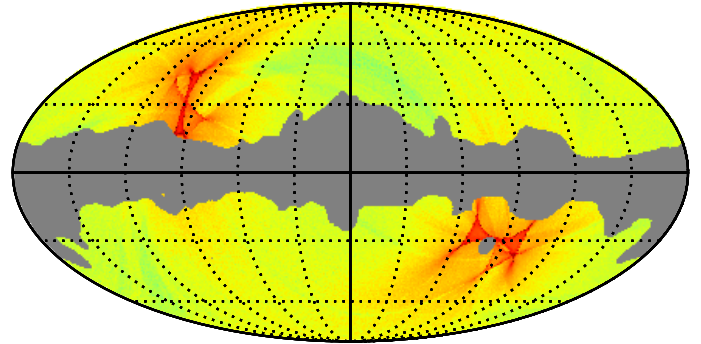
1 Hit count 20000 Random selection
