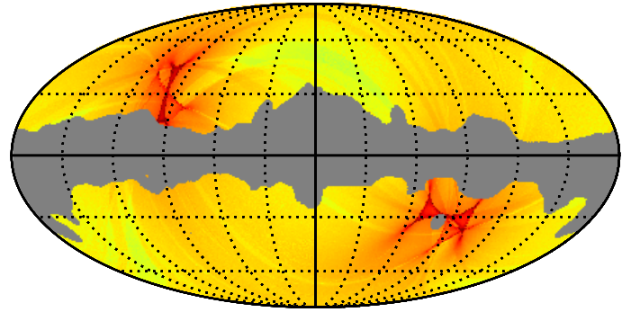
1 Hit count 20000 Superclean selection
