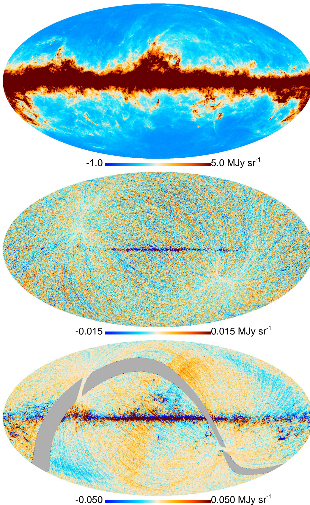
Figure 19. HFI maps at 545 GHz. The top panel gives the intensity in \text{MJy sr}^{-1} . The middle panel shows the difference between maps made from the first and the second halves of each stable pointing period (i.e., half-ring maps). The bottom panel shows the difference between Survey 1 and Survey 2.
