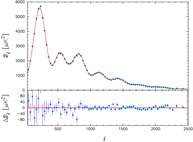
Figure 15. Top: Planck maximum-likelihood (primary) CMB spectrum compared with the best-fit six parameter \Lambda\text{CDM} spectrum. Bottom: Power spectrum residuals with respect to the \Lambda\text{CDM} model. The error bars are computed from the diagonal elements of the band-averaged covariance matrix, as given by Eq. A.25, including contributions from foreground and beam transfer function errors.
