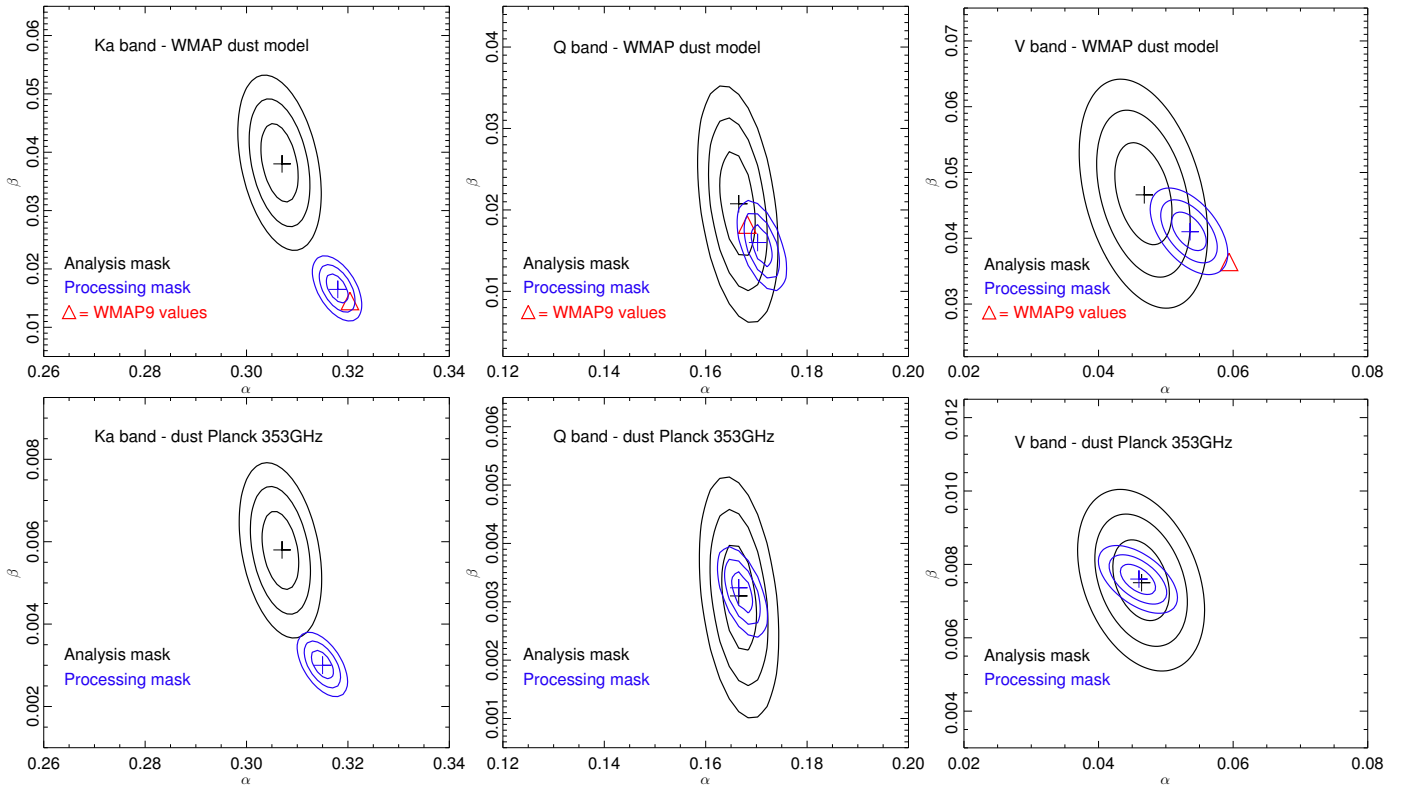
Figure E.1. 1 \sigma and 2 \sigma contours for the template coefficient scalings estimated using the WMAP dust template ( top ) and the Planck 353 GHz map as a dust template ( bottom ), for the Ka, Q, and V bands. We compare the coefficients estimated using the WMAP ‘P06’ mask, to this with the smaller WMAP ‘processing mask’. We also indicate the template values quoted in the WMAP paper Bennett et al. (2012) .
