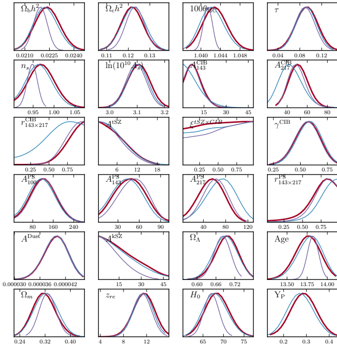
Figure 27. Posterior distributions for cosmological parameters, varying the Helium abundance Y_P (red). We show the effect of marginalizing over calibration and beam errors (blue), and the results obtained using the reference settings (purple), where Y_P is constrained by BBN.
