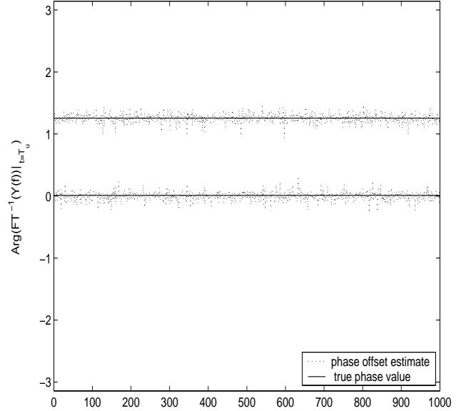
Figure 1: \Phi_{f_c}^1 estimation for \Delta f_c = 0 and \Delta f_c = 1/5T_u . AWGN channel with SNR = 10dB .
