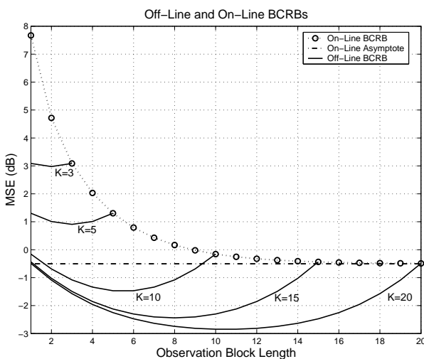
Fig. 1. BCRBs versus the number of observations for \sigma_n^2 = 4 , \sigma_w^2 = 0.16 \text{ rad}^2 ( J_D is evaluated over 10^5 Monte-Carlo trials).
