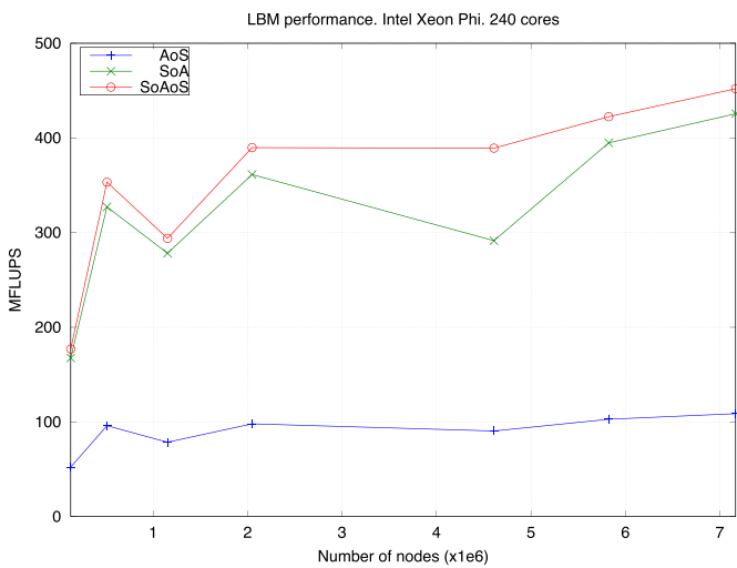
(b) 240 threads
