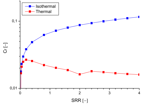
Figure 5: Variation of the friction coefficient as a function of the slide-to-roll ratio (SRR) for the reference configuration (see Table 1).
