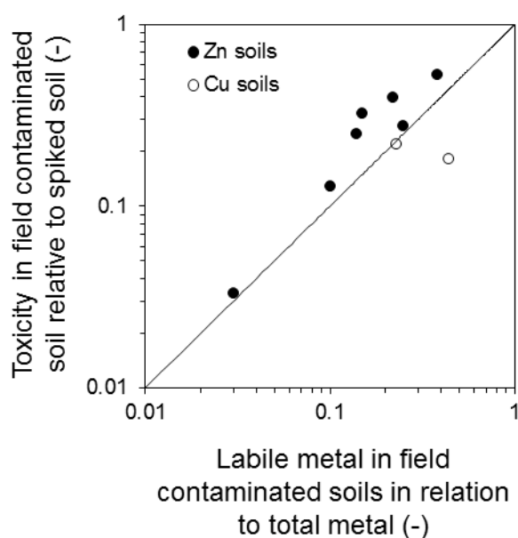
Figure 5.6 Labile metal fraction in the field-contaminated soil (fraction of aqua regia soluble metal that is isotopically exchangeable) plotted versus the relative metal toxicity (expressed as the ratio between the EC50 of the spiked soil and the EC50 field-contaminated soil). The 1:1 line is indicated, ( r=0.82 on log-log plot).
