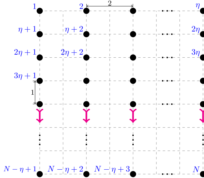
Fig. 1. A regular N -node multiline grid network.
