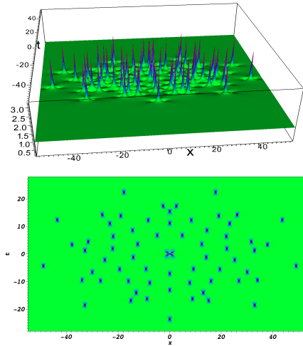
Figure 9: Solution of NLS, N=11 , \tilde{b}_4 = 10^9 : 6 rings with 9; 9; 18; 9; 9; 9 peaks, with in the center P_2 ; in bottom, sight of top.
