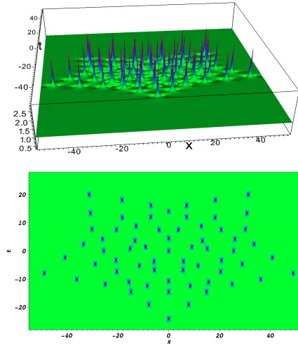
Figure 5: Solution of NLS, N=11 , \tilde{b}_2 = 10^5 : 9 rings with 5; 10; 10; 5; 5; 10; 5 : 10; 5 peaks, with in the center one peak; in bottom, sight of top.
