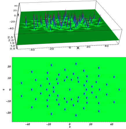
Figure 12: Solution of NLS, N=11 , \tilde{a}_6 = 10^{13} : 5 rings with 13 peaks and in the center one peak; in bottom, sight of top.
