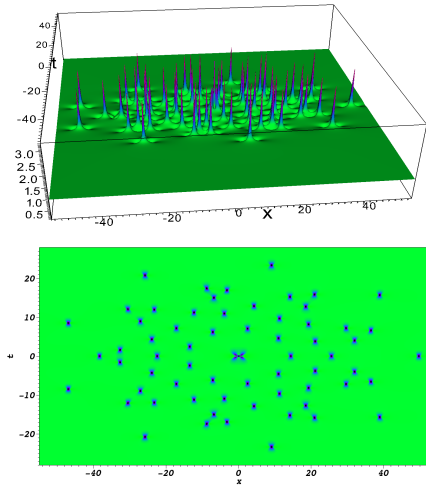
Figure 8: Solution of NLS, N=11 , \tilde{a}_4 = 10^9 : 6 rings with 9; 9; 18; 9; 9; 9 peaks, with in the center P_2 ; in bottom, sight of top.
