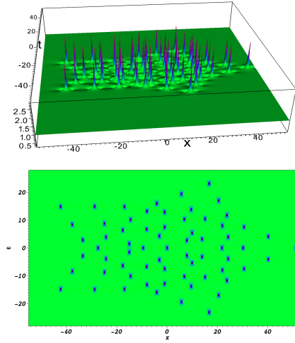
Figure 4: Solution of NLS, N=11 , \tilde{a}_2 = 10^5 : 9 rings with 5; 10; 10; 5; 5; 10; 5 : 10; 5 peaks, with in the center one peak; in bottom, sight of top.
