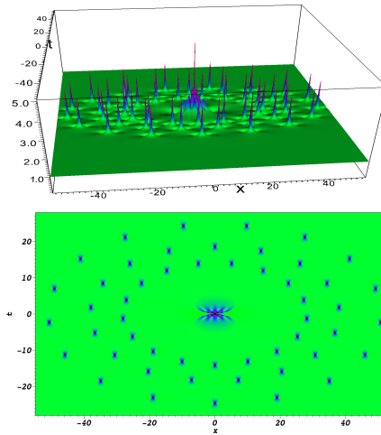
Figure 17: Solution of NLS, N=10 , \tilde{b}_8 = 10^{18} : 3 rings with 17 peaks and in the center the Peregrine breather of order 5; in bottom, sight of top.
