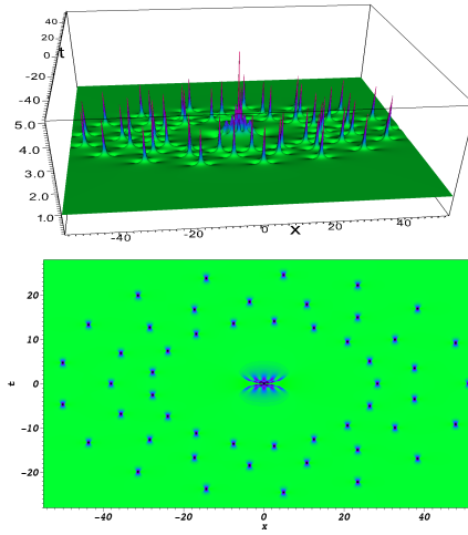
Figure 16: Solution of NLS, N=11 , \tilde{a}_8 = 10^{18} : 3 rings with 17 peaks and in the center the Peregrine breather of order 5; in bottom, sight of top.
