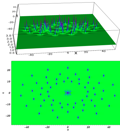
Figure 15: Solution of NLS, N=11 , \tilde{b}_7 = 10^{15} : 4 rings with 15 peaks and in the center the Peregrine breather of order 3; in bottom, sight of top.
