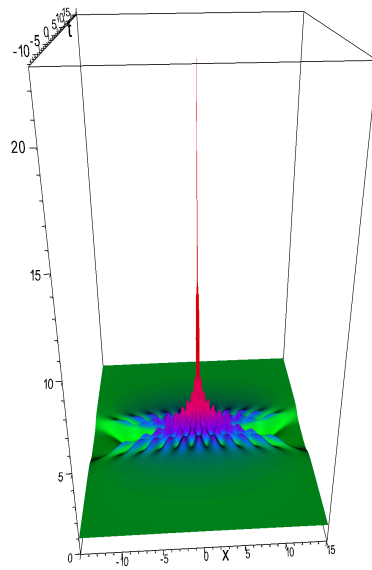
Figure 1: Solution of NLS, N=11, all parameters equal to 0, Peregrine breather P_{11} .
