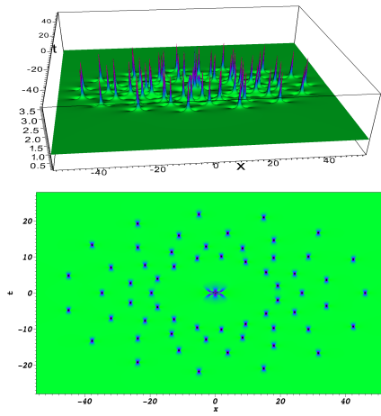
Figure 14: Solution of NLS, N=11 , \tilde{a}_7 = 10^{15} : 4 rings with 15 peaks and in the center the Peregrine breather of order 3; in bottom, sight of top.
