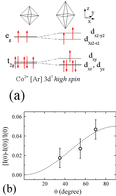
Figure 4: (a) Schematic figure of the 3d orbital occupancy for \text{Co}^{2+} in octahedral environment. For the axial elongation of the point charge octahedron along z , the degeneracy of the t_{2g} orbitals is lifted and the lowest level unpaired electron lies in the d_{xy} orbital; (b) experimental angular variation of the integrated intensity of the XAS spectra (dots). The dotted line corresponds to the calculated I_{xy}(\theta) function.
