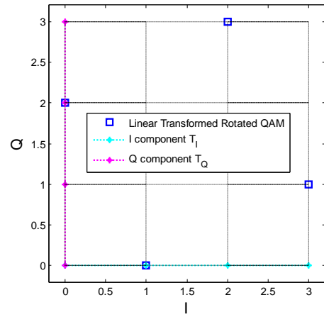
Fig.2. Linear transformed rotated QPSK (T_i, T_\ell) from (z_i, z_\ell) by using (12) and (13).
