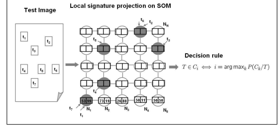
Figure 4. Decision rule.
