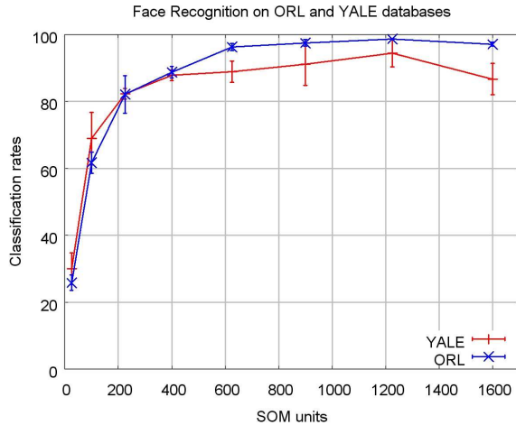
Figure 6. Face recognition results.
