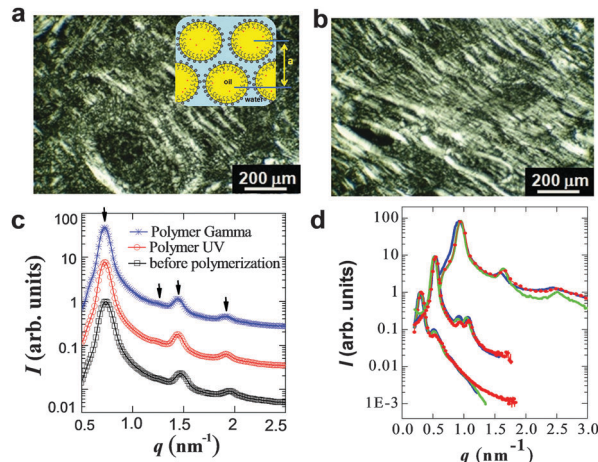
Fig. 1 Representative polarized light micrographs of hexagonal mesophases (a) before and (b) after photopolymerization ( \phi = 2.21 , C_s = 0.3 \text{ mol L}^{-1} ). Inset of a: Cross section of swollen hexagonal mesophases, a is the lattice parameter of hexagonal mesophases. (c) SAXS spectra of swollen hexagonal phases before polymerization ( \square ) and after polymerization by UV irradiation ( \circ ), gamma irradiation ( * ) at 0.1 M NaCl ( \phi = 0.98 ). The arrows specify the indexing of the Bragg peaks. (d) Representative SAXS spectra of swollen hexagonal phases with various swelling ratios and salt concentrations from top to bottom (top, \phi = 0.22 , C_s = 0 \text{ mol L}^{-1} with less oil, middle, \phi = 0.72 with relatively more oil, C_s = 0 \text{ mol L}^{-1} , bottom, \phi = 2.21 , C_s = 0.3 \text{ mol L}^{-1} ). Before polymerization (blue line), after polymerization by UV light irradiation (red line), and gamma irradiation (green line).
