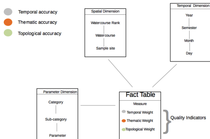
Figure 4: Spatial quality data warehouse star schema: a measure is a tuple \langle \text{parameter, unit, value, date, sample site} \rangle
