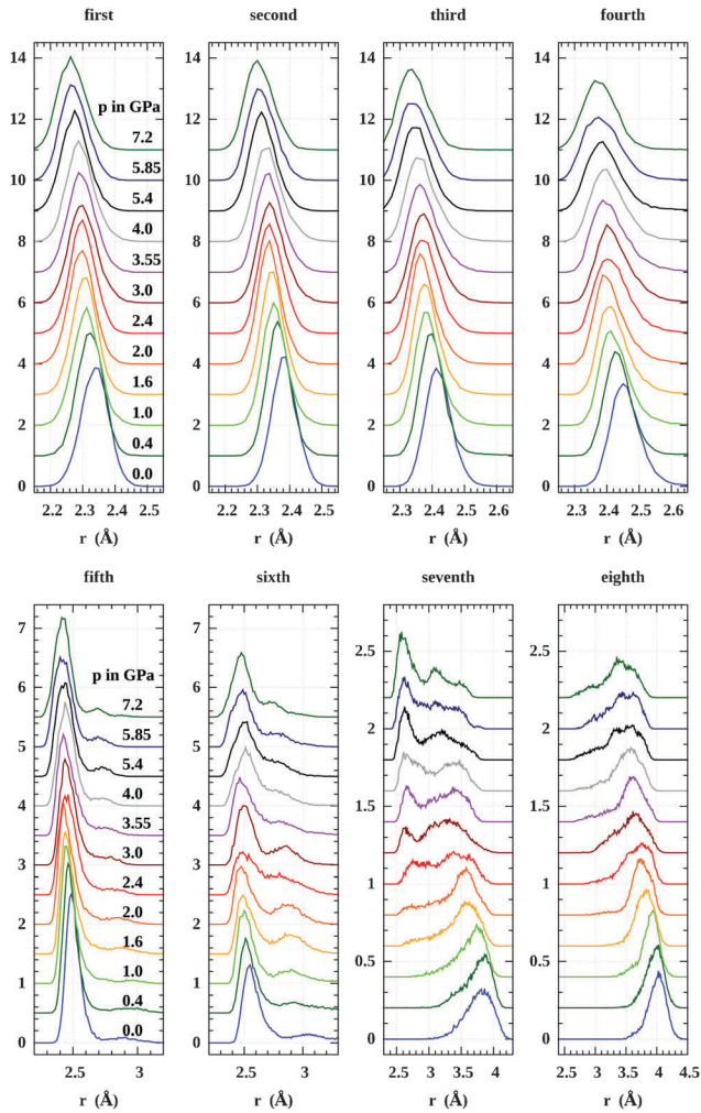
Fig. 8 Evolution with pressure of the distance distribution of the eight closest neighbours (O and Cl - ) to Na + ions, where r is the distance to the sodium ion. The seventh and eighth neighbours move into the shell of first neighbours above 2 GPa.
