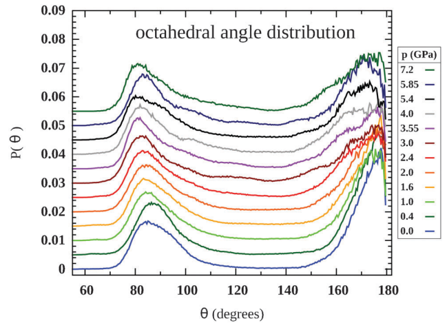
Fig. 9 Evolution with pressure of the distribution of octahedral angles, which are the angles at the central Na + ion between atoms at the corners of the octahedron formed by the six nearest neighbours.
