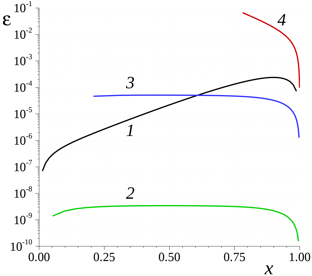
Figure 2. Distribution of the numerical error in the computational domain for various choices of the monitor function \omega(x) : (1) — \omega(x) \equiv 1 (i.e. the uniform grid), (2) — \omega(x) = (u_x(x))^{\frac{1}{4}} (optimal case), (3) — \omega(x) = (u_x(x))^{\frac{1}{2}} , (4) — \omega(x) = (u_x(x))^2 . The problem parameters are \ell = 1 , \lambda = 10 and only N = 80 nodes are used.
