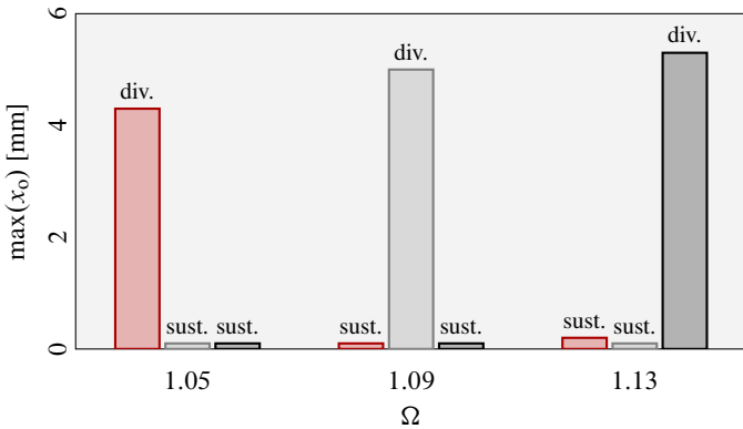
Figure 24. Maximal shaft displacements near \Omega_1^{\text{cr}} : \kappa = 0 \text{ N/m} [red], \kappa = 500 \text{ N/m} [black] and \kappa = 1000 \text{ N/m} [grey]
