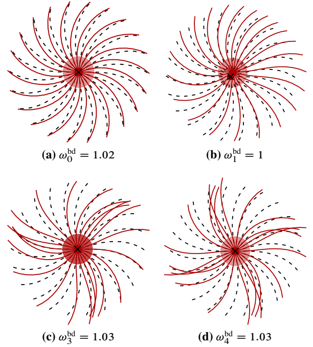
Figure 6. First family of free vibration modes: center node displaced [●] and rest [✕] position
