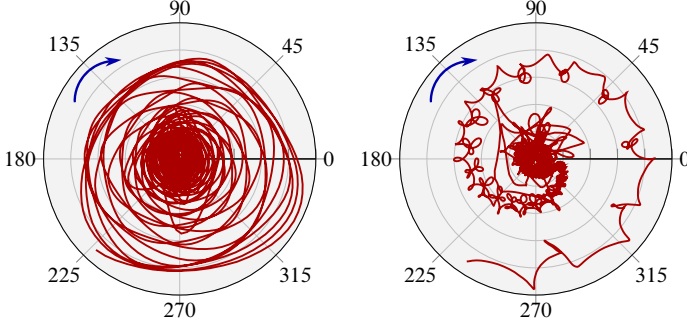
(a) Rotating frame: backward precession (b) Static frame: almost no precession as \Omega_1^{cr} is very close to \omega_1^{bd}
