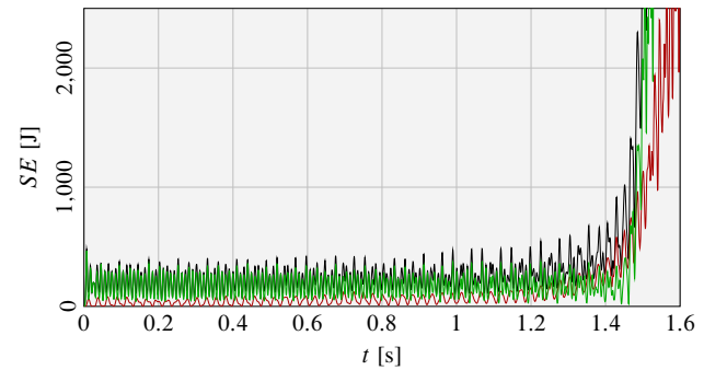
Figure 26. Strain energy for \kappa = 0 \text{ N/m} at \Omega = 1.65 : total [black], k = 1 [red] and susp. [green]
