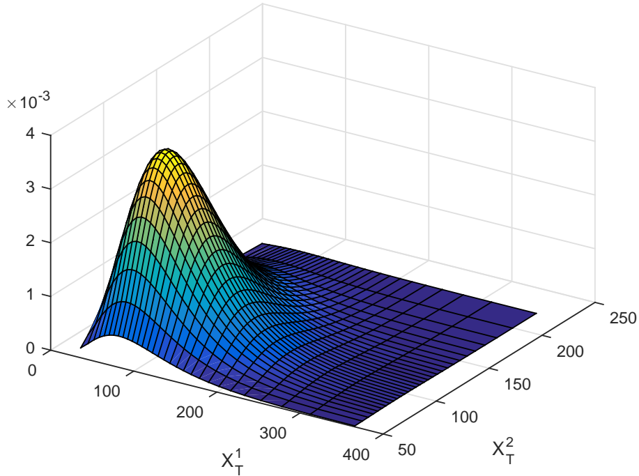
Figure 1: Distribution of the weights in the uncorrelated case at time t = T, N^1 = N^2 = 30 .
