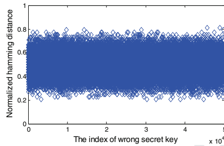
Fig. 8. Distribution of normalized Hamming distance when using 50000 wrong secret keys
