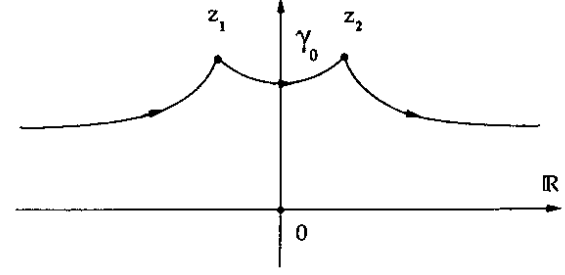
Figure 5: The dissipative path \gamma_0 .
