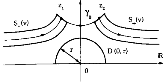
Figure 6: The disc D(0, r) and the tubular neighbourhoods S_-(v) and S_+(v) of \gamma_0 .
