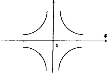
Figure 4: The level lines \text{Im}z^2 = \text{cst} .
