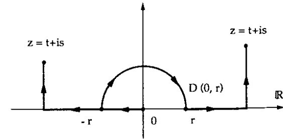
Figure 7: Particular integration paths.
