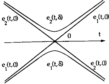
Figure 1: The levels e_j(t, \delta) and e_j(t, 0) .
