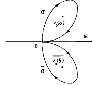
Figure 3: The integration path \sigma \cup \bar{\sigma} .
