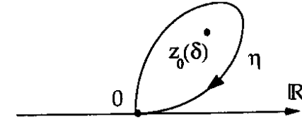
Figure 2: The loop \eta and the eigenvalue crossing z_0(\delta) .
